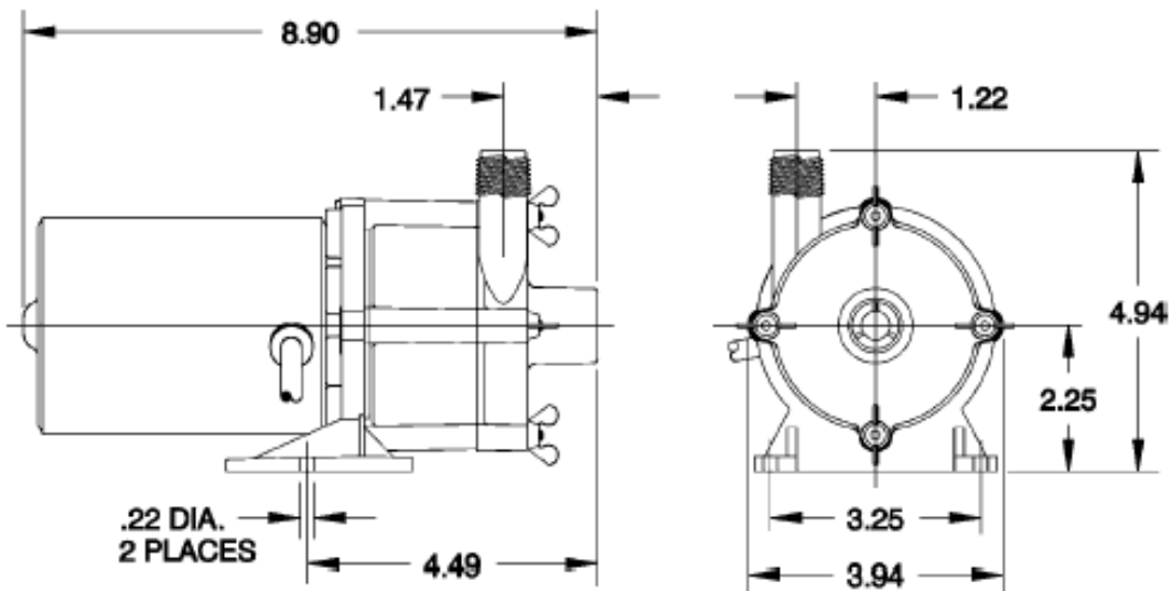
SPEC OF 3MD-HC PUMP
